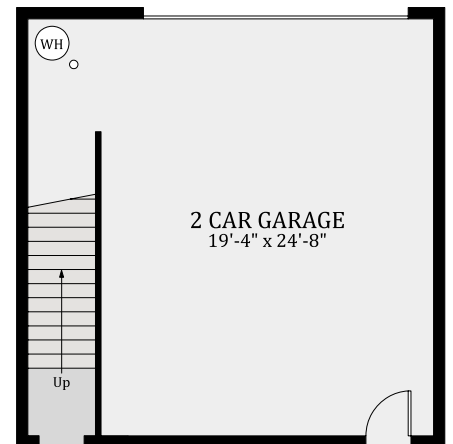
OPTIONAL EXPANDED 2 CAR GARAGE W/ APARTMENT COURTYARD ACCESS
