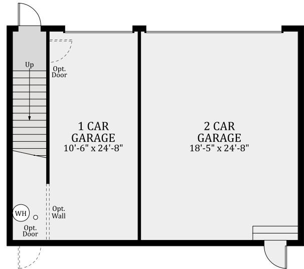
OPTIONAL SPLIT GARAGE W/ APARTMENT ALLEY ACCESS
