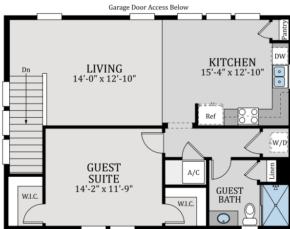
OPTIONAL 3 CAR GARAGE APARTMENT W/ COURTYARD ACCESS AND BREEZEWAY
