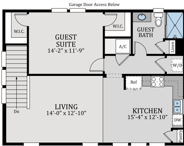
OPTIONAL 3 CAR GARAGE APARTMENT W/ ALLEY ACCESS AND BREEZEWAY
