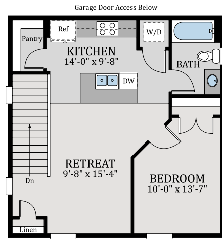
OPTIONAL EXPANDED 2 CAR GARAGE APARTMENT W/ ALLEY ACCESS
